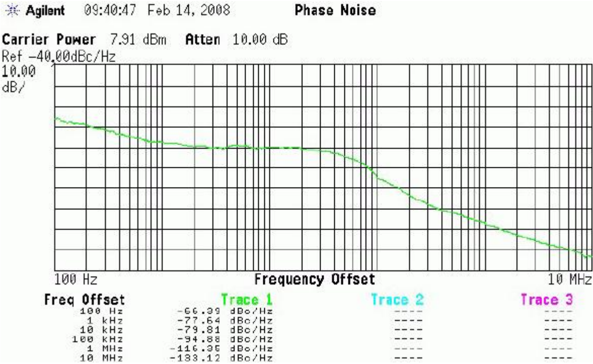
Figure 41. Synthesizer Phase Noise (VCOCURR = 11)
