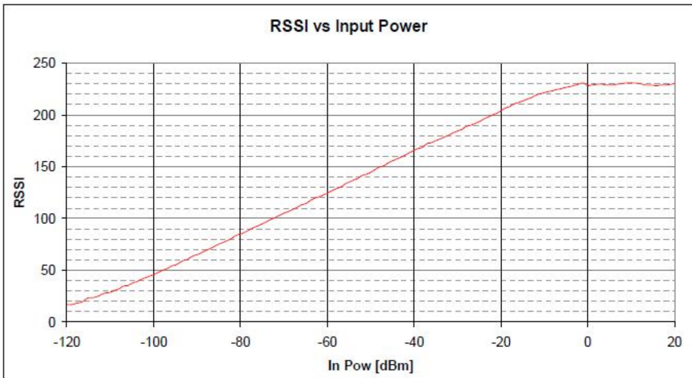
Figure 30. RSSI Value vs. Input Power
