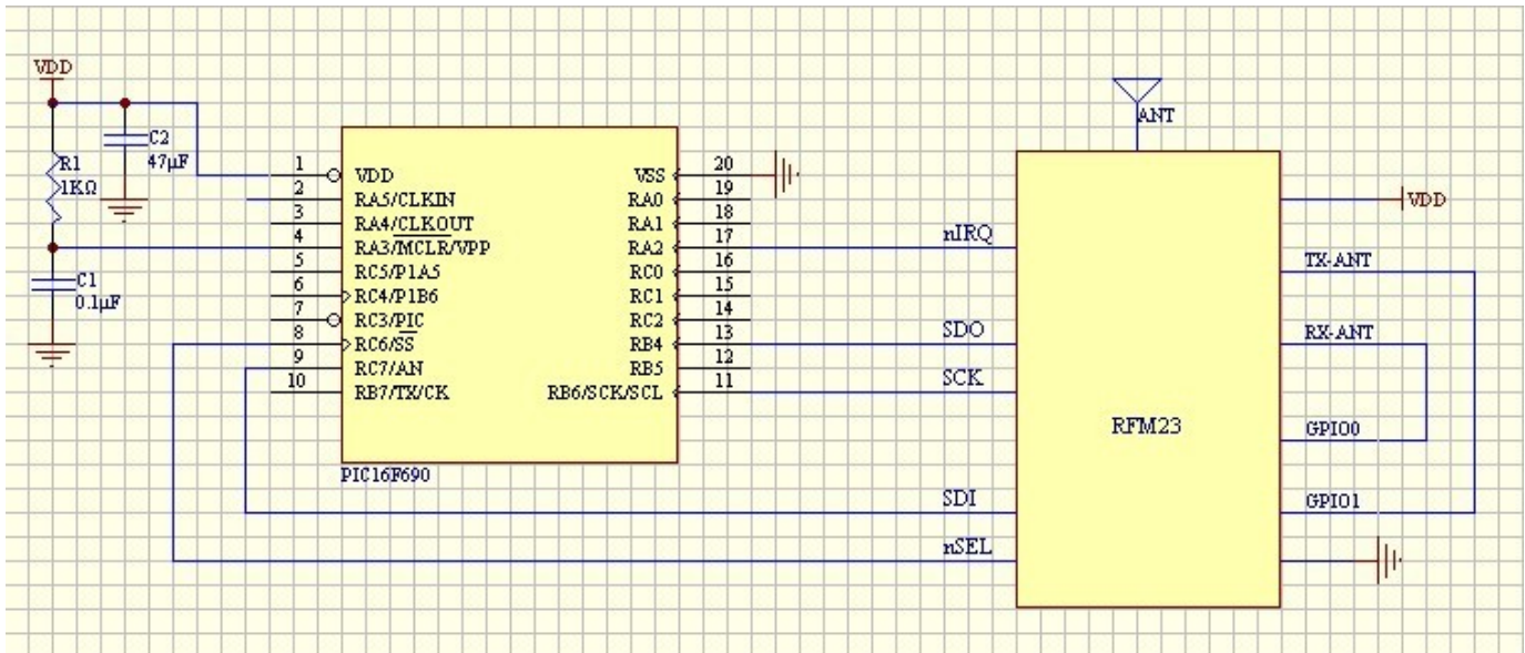
RFM23 Reference Design Schematic 1
