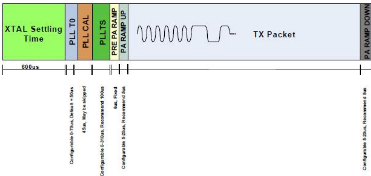
Figure 7. TX Timing
