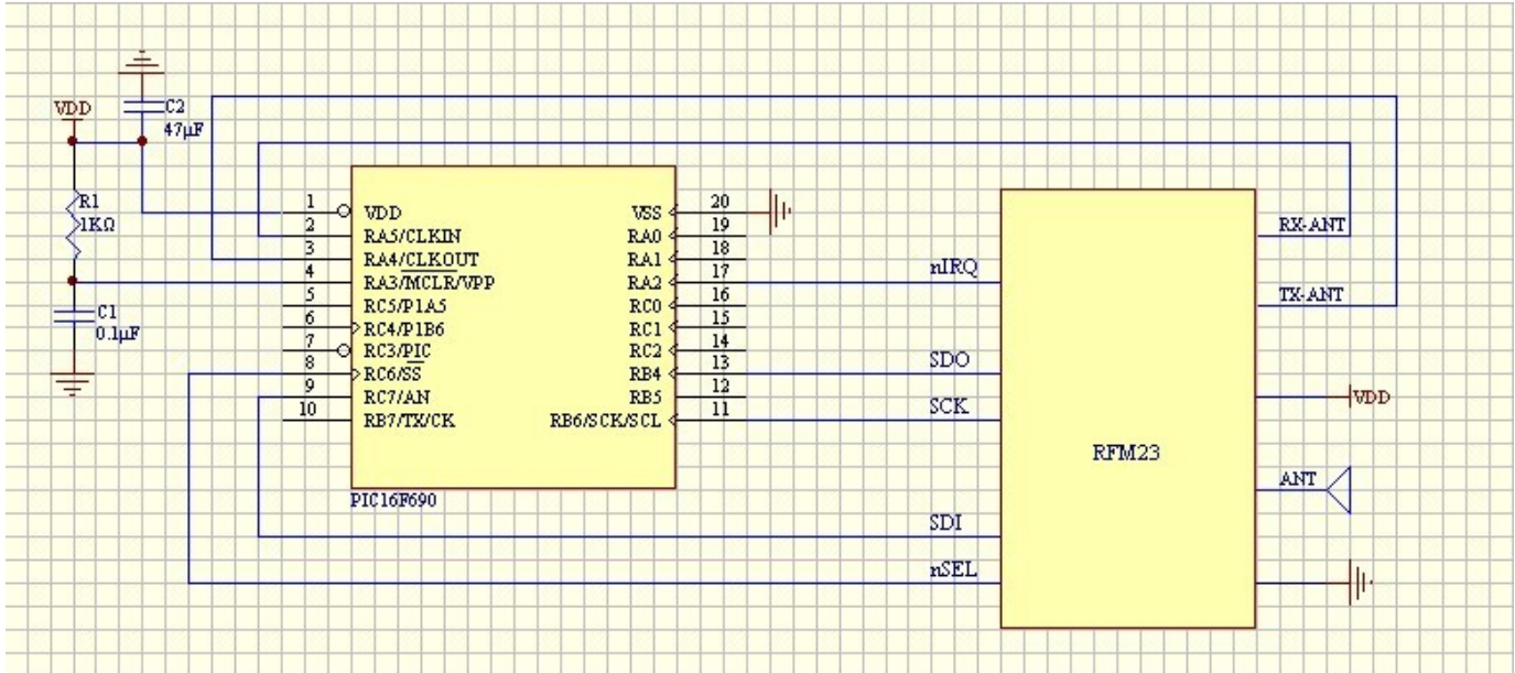
RFM23 Reference Design Schematic 1
