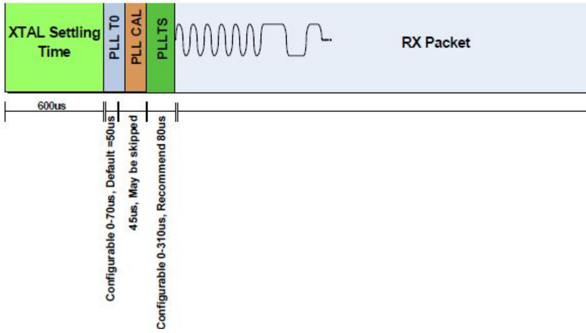
Figure 8. RX Timing
