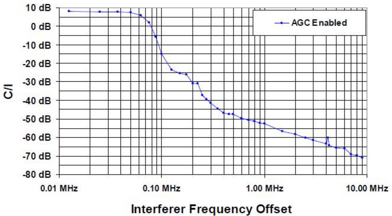
Figure 36. Receiver Selectivity
