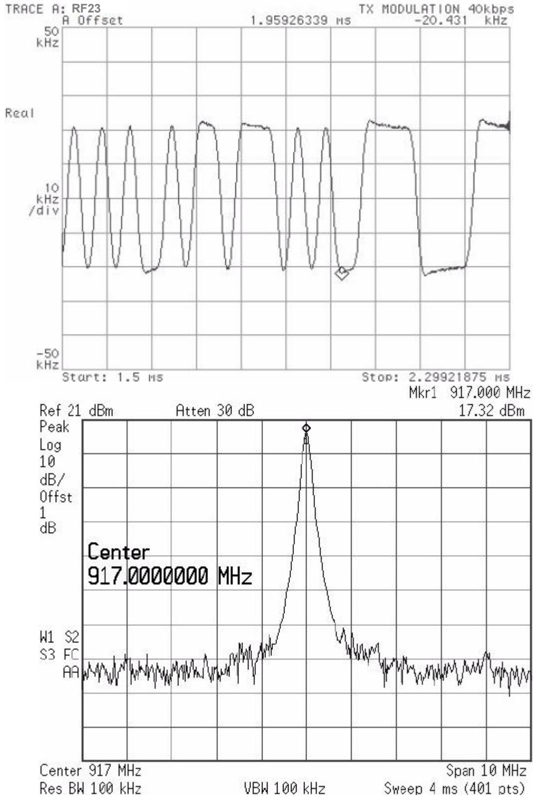
Figure 38. TX Unmodulated Spectrum (917 MHz)
